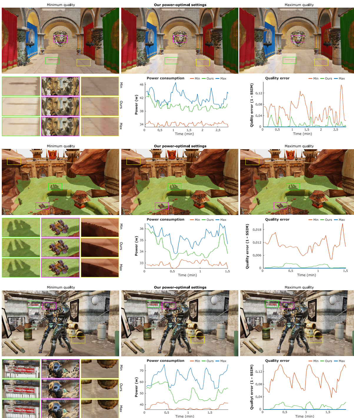
Figure 11: Sponza (top), Valley (middle) and Subway (bottom) demo scenes, executed on a desktop PC. We compare the minimum and maximum quality rendering configurations against our power-optimal configuration. For Sponza, we use a power budget of 60% (which corresponds to a percentage of the difference between the Min and Max power consumptions); for Valley we use 40%, and for Subway we use 50%. Our method generates images very similar to those rendered with the maximum quality configuration, while keeping power consumption lower. Please refer to the supplementary video for the full demos.
