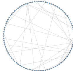
Watts-Strogatz
