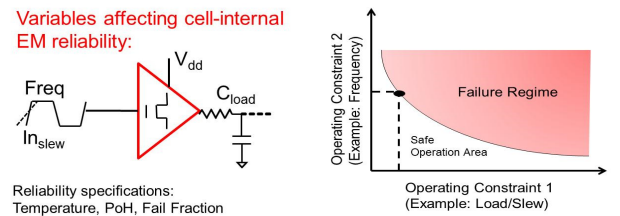
Fig. 2 (a): Variables affecting cell-internal EM. (b): Traditional EM verification using the safe operating region concept.
