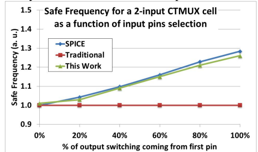
Fig. 4. f_{safe} for the circuit in Fig. 3, at selected load/slew. f_{safe} varies based on the extent of switching coming from first or second pin. The proposed model captures the behavior fully, unlike the excessively pessimistic traditional one.
