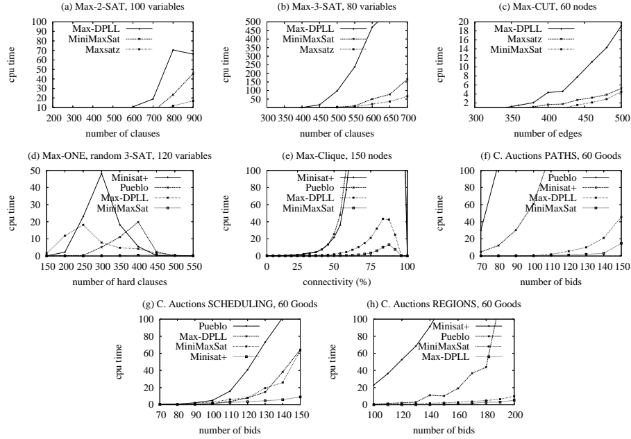
Fig. 2. Plots of different benchmarks.
