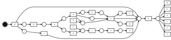
(c) Simplified series-parallel process model.
