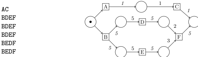
(a) Example trace (b) Petri net with trigger/utilization scores
